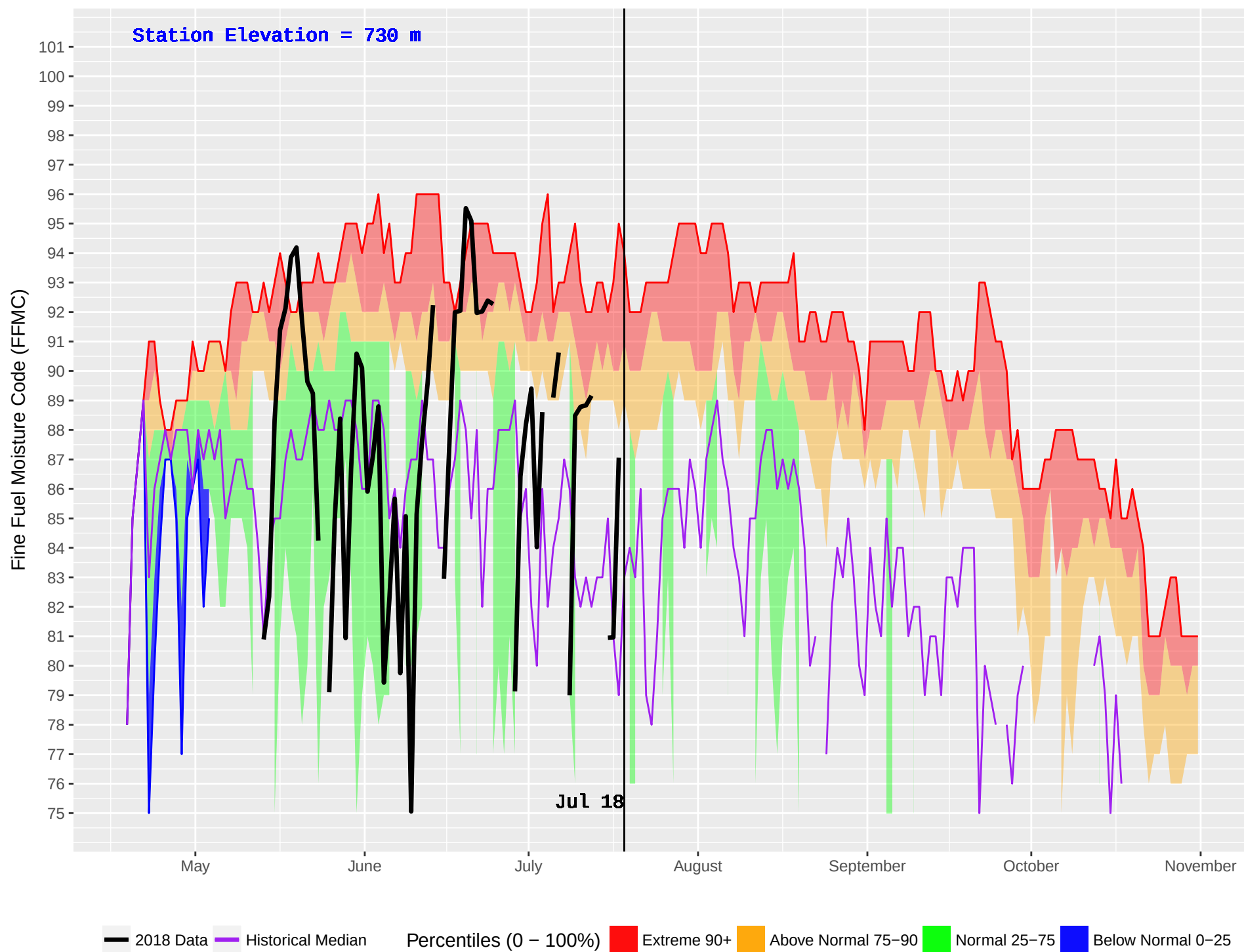
BOYA LAKE (445) : Historical (1985–2016) and Current (2018) Daily Fine Fuel Moisture Code (FFMC)
